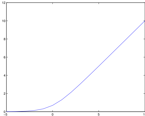
Figure 2.5: Rectified linear units. The figure shows \log(1 + e^x) .
